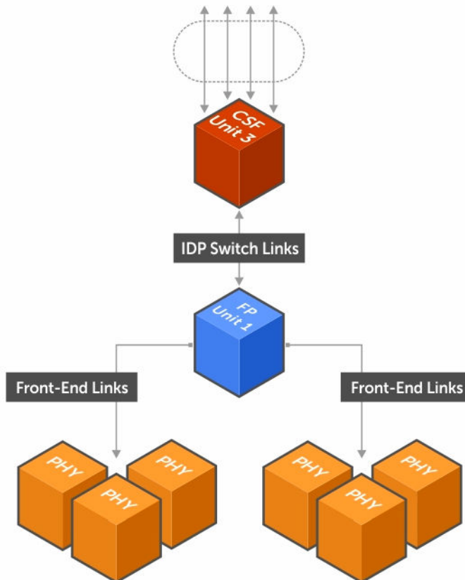
Figure 130. Buffer Tuning Points
